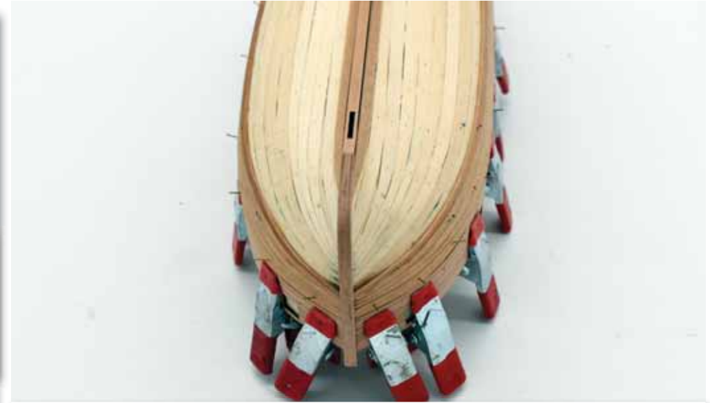
Planking progress at bow (above) and stern (below). If you do not get the end planks at the stern perfectly butted up against the stern counter, do not worry too much, as this line is covered by stern counter rails (124 and 125)
