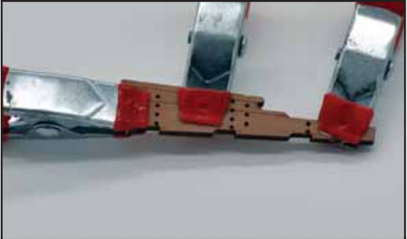
84. The main rudder assembly consists of three parts, the core (90), the right side (91) and left (92). 91 and 92 are glued to 90.
