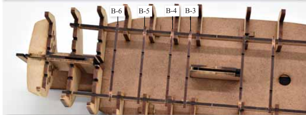
20. Slot and glue B-3, B-4, B-5 and B-6 into position. The positions of each part can also be found on Plan Sheet 3
