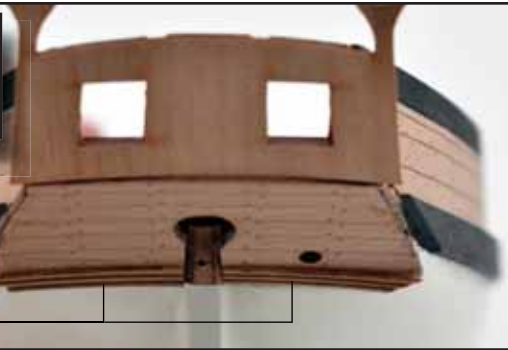
74. Remove the stern transom (83) from the 1.5mm wood sheet and glue in place, as shown. Again, this can be clamped until the glue has cured. Once cured, file the openings so both layers are completely flush with one another.
